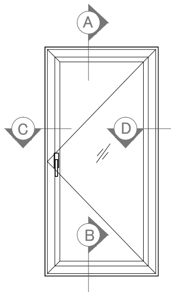
ELEVATION OUTSIDE VIEW
