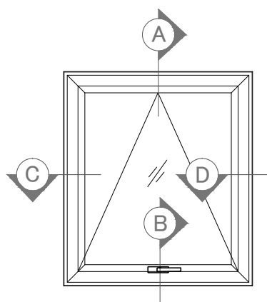
ELEVATION OUTSIDE VIEW
