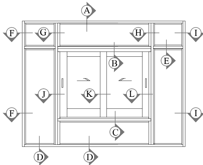
ELEVATION OUTSIDE VIEW
